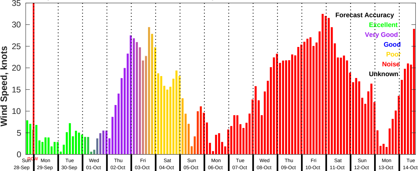
GFS Wind Speed Forecast for NDBC 46028 from 28-Sep-2025 16:00:00 to 14-Oct-2025 16:00:00
