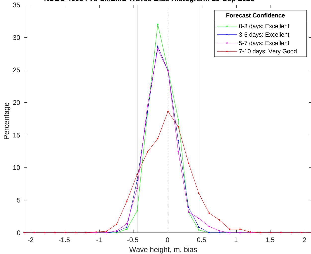
NDBC 46054 vs CMEMS Waves Bias Histogram: 29-Sep-2025
