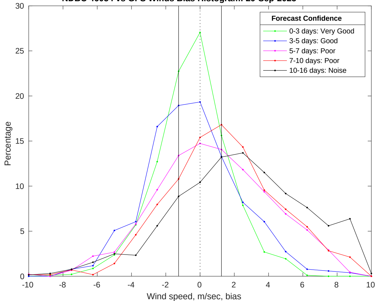
NDBC 46054 vs GFS Winds Bias Histogram: 29-Sep-2025
