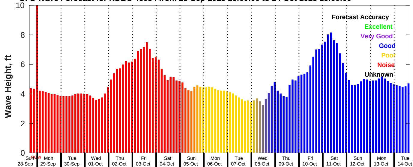
GFS Wave Forecast for NDBC 46054 from 28-Sep-2025 16:00:00 to 14-Oct-2025 16:00:00
