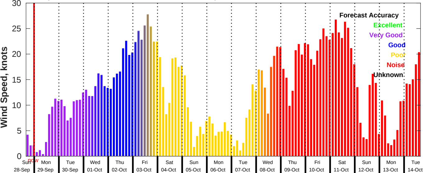
GFS Wind Speed Forecast for NDBC 46054 from 28-Sep-2025 16:00:00 to 14-Oct-2025 16:00:00
