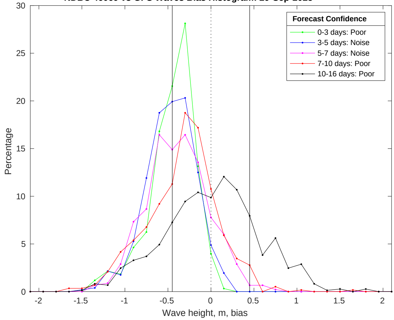
NDBC 46069 vs GFS Waves Bias Histogram: 29-Sep-2025
