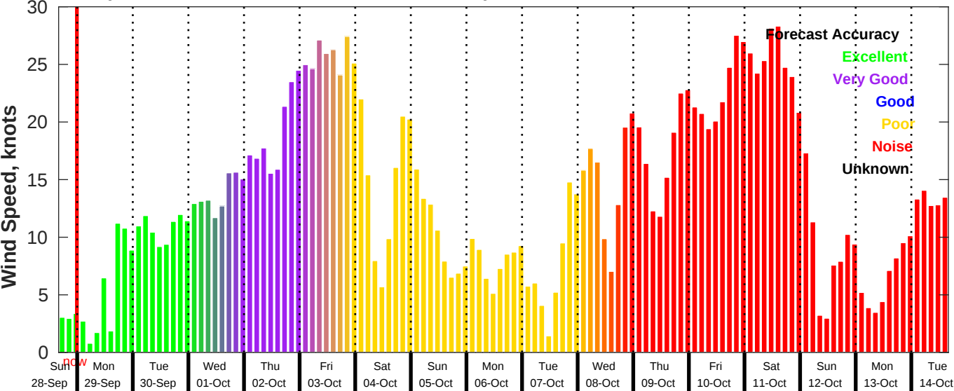
GFS Wind Speed Forecast for NDBC 46069 from 28-Sep-2025 16:00:00 to 14-Oct-2025 16:00:00
