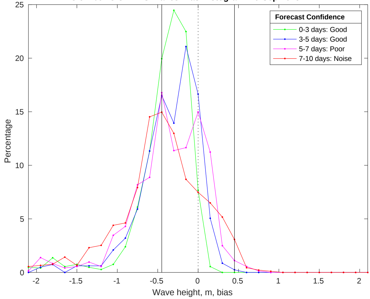
NDBC 51209 vs CMEMS Waves Bias Histogram: 29-Sep-2025
