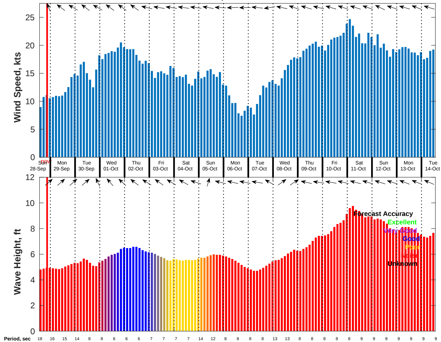
Wind & Wave Forecast for NDBC 51209 from 28-Sep-2025 13:00:00 to 14-Oct-2025 13:00:00
