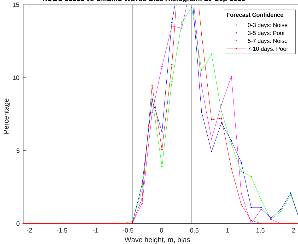
NDBC 51211 vs CMEMS Waves Bias Histogram: 29-Sep-2025
