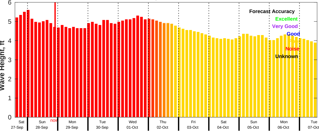
CMEMS Wave Forecast for NDBC 51211 from 27-Sep-2025 14:00:00 to 07-Oct-2025 14:00:00
