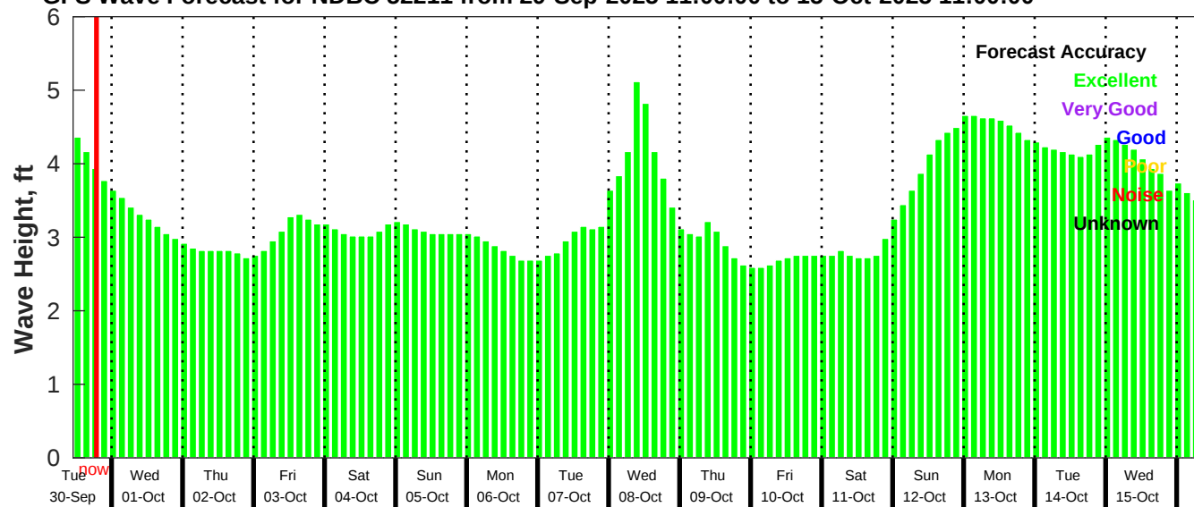
GFS Wave Forecast for NDBC 52211 from 29-Sep-2025 11:00:00 to 15-Oct-2025 11:00:00
