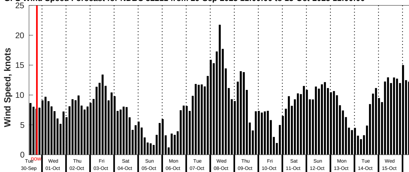
GFS Wind Speed Forecast for NDBC 52211 from 29-Sep-2025 11:00:00 to 15-Oct-2025 11:00:00
