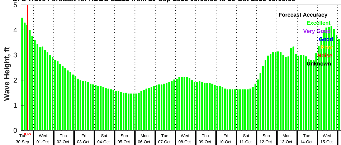
GFS Wave Forecast for NDBC 52212 from 29-Sep-2025 09:00:00 to 15-Oct-2025 09:00:00
