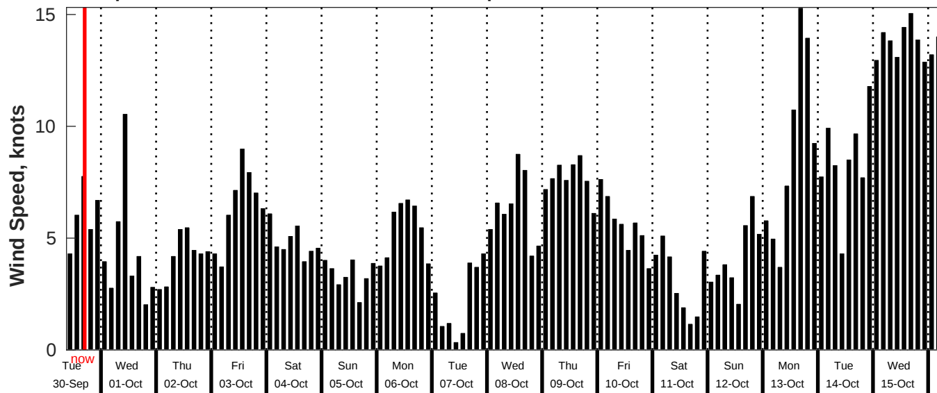
GFS Wind Speed Forecast for NDBC 52212 from 29-Sep-2025 09:00:00 to 15-Oct-2025 09:00:00
