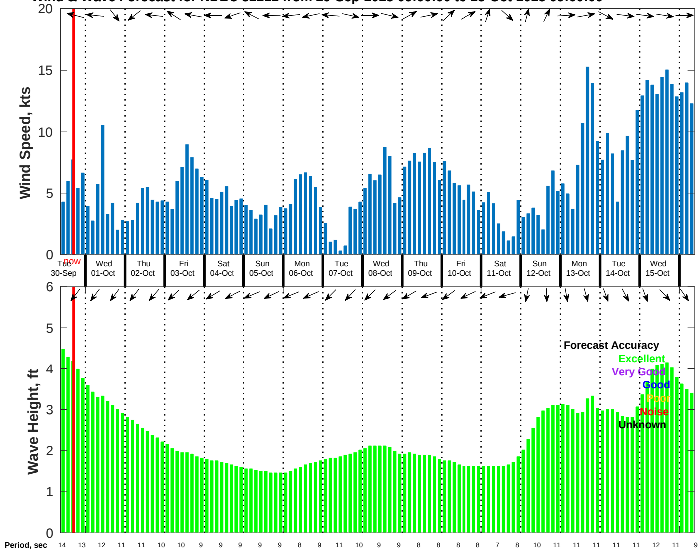
Wind & Wave Forecast for NDBC 52212 from 29-Sep-2025 09:00:00 to 15-Oct-2025 09:00:00
