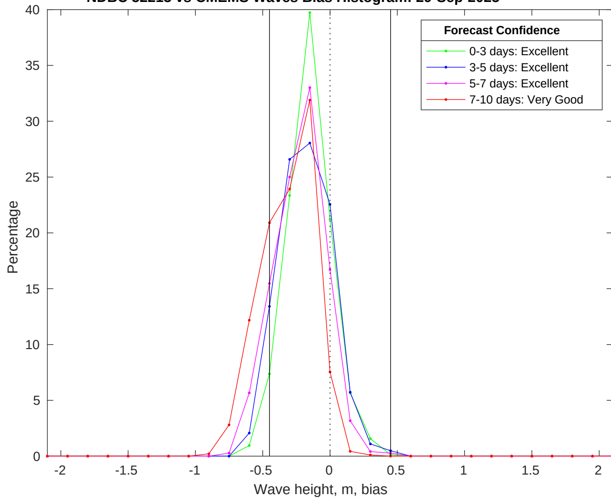
NDBC 52213 vs CMEMS Waves Bias Histogram: 29-Sep-2025
