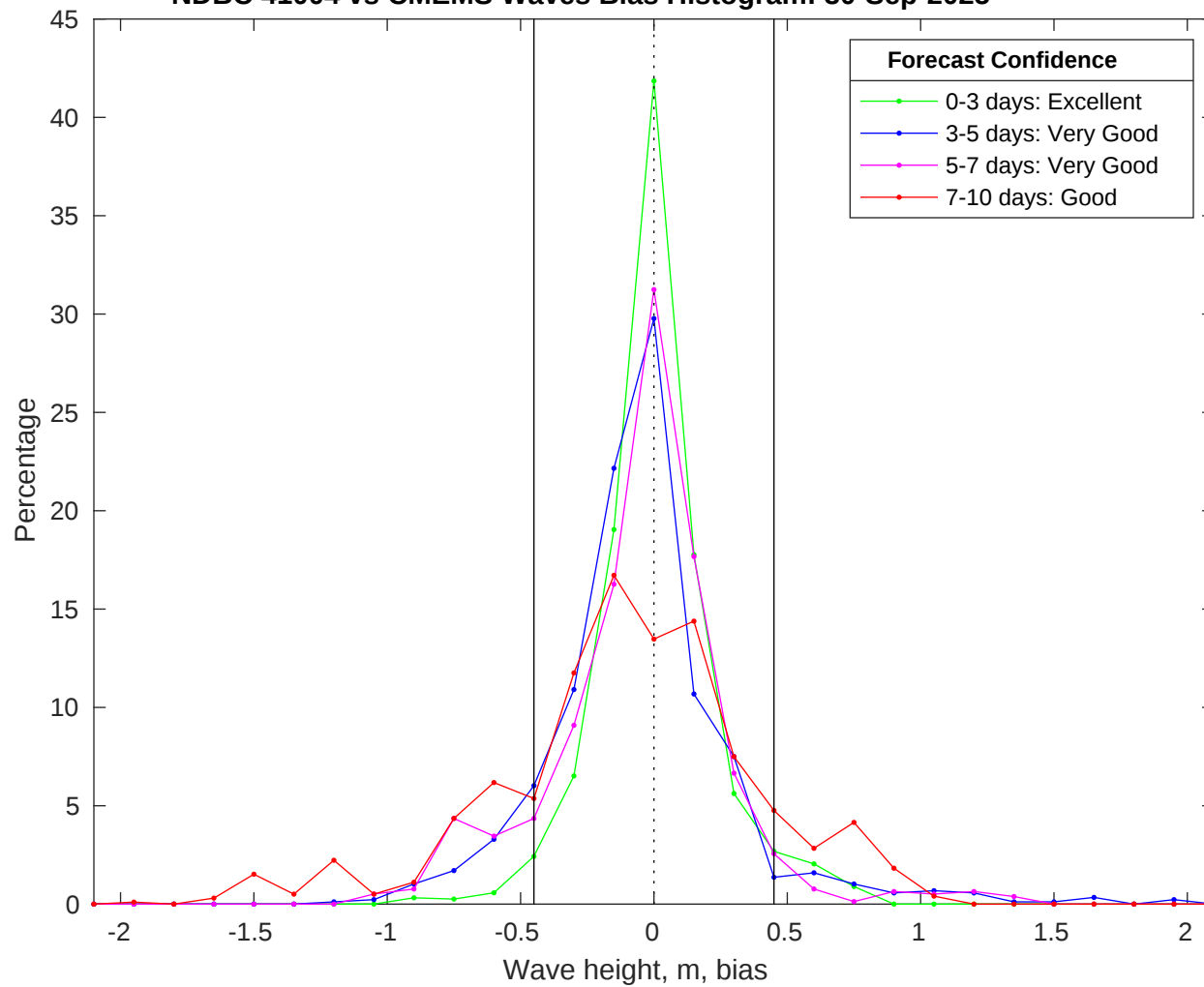
NDBC 41004 vs CMEMS Waves Bias Histogram: 30-Sep-2025
