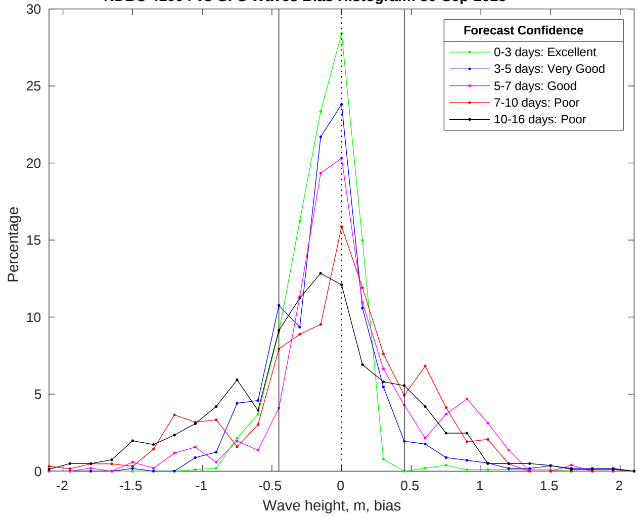
NDBC 41004 vs GFS Waves Bias Histogram: 30-Sep-2025
