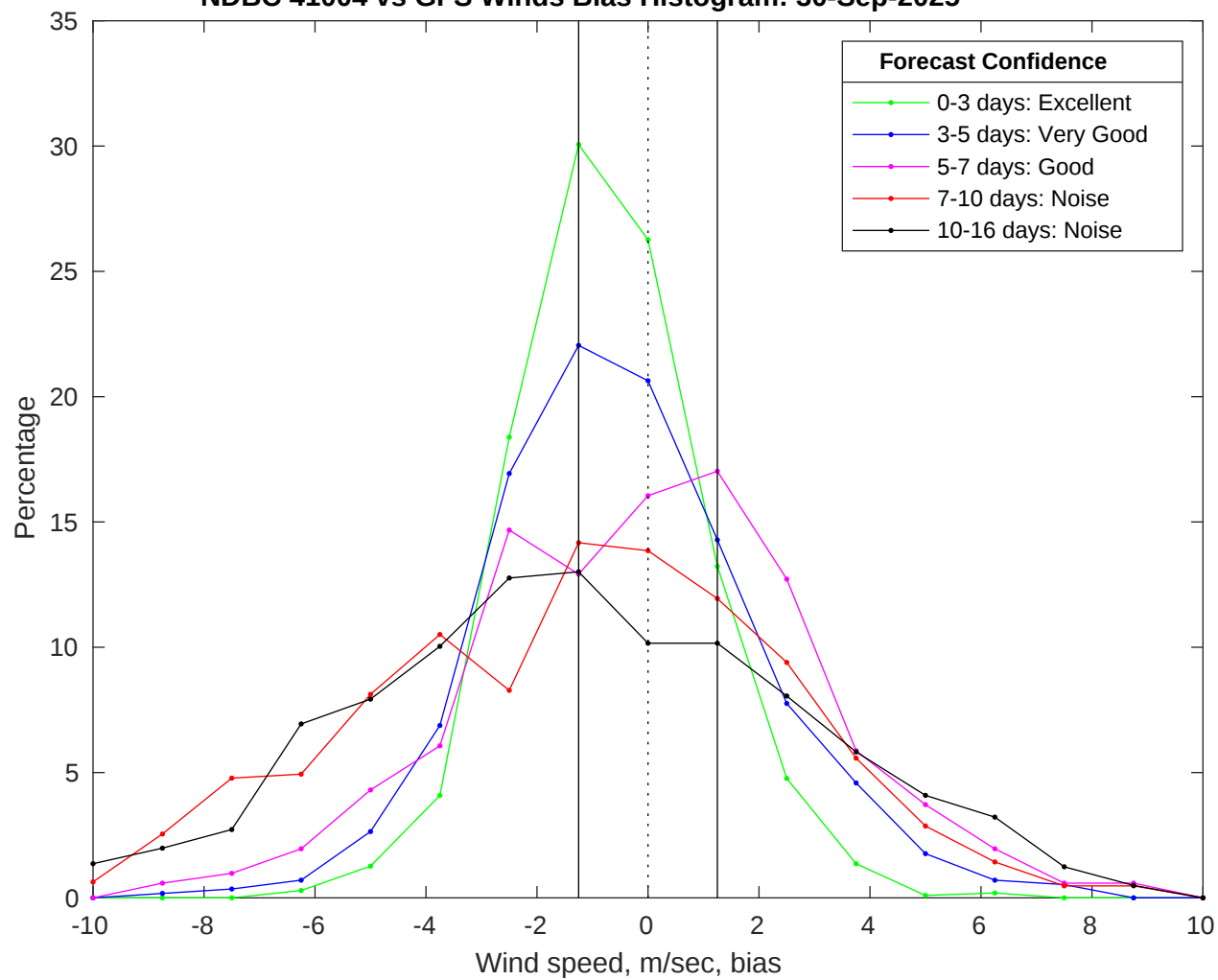
NDBC 41004 vs GFS Winds Bias Histogram: 30-Sep-2025
