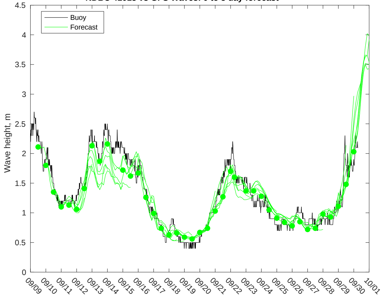
NDBC 41013 vs GFS Waves: 0 to 3 day forecast
