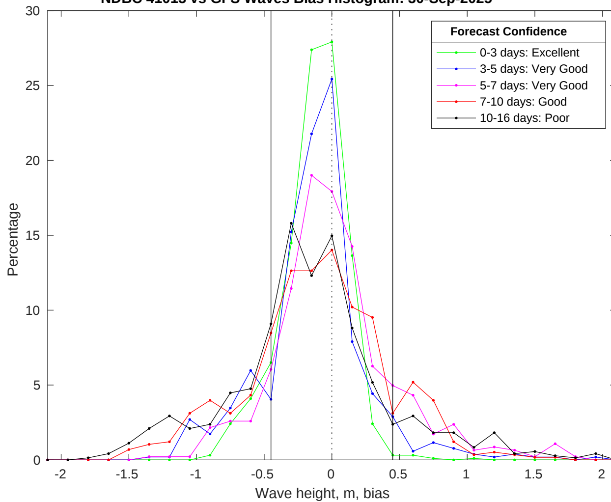
NDBC 41013 vs GFS Waves Bias Histogram: 30-Sep-2025
