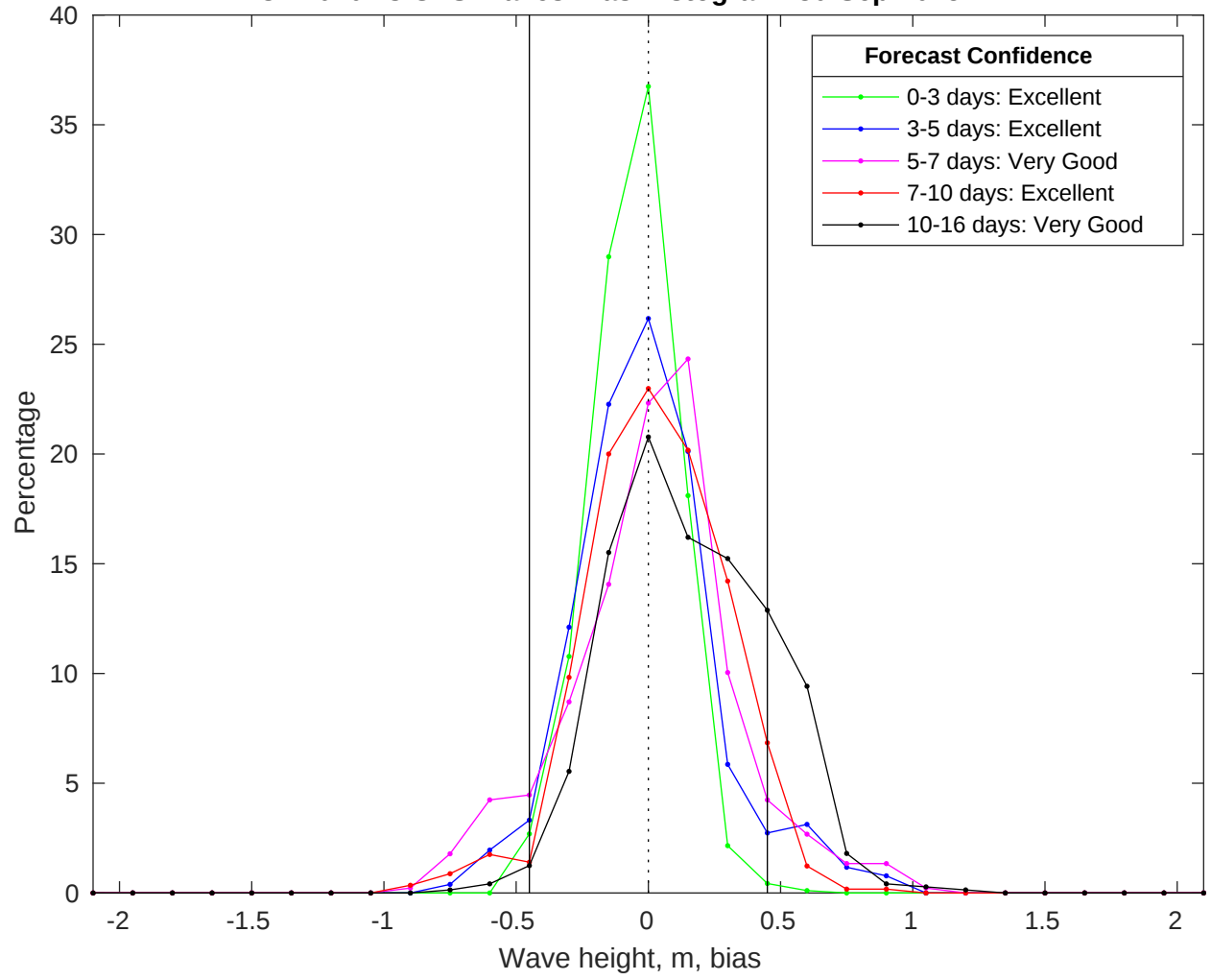
NDBC 41040 vs GFS Waves Bias Histogram: 30-Sep-2025
