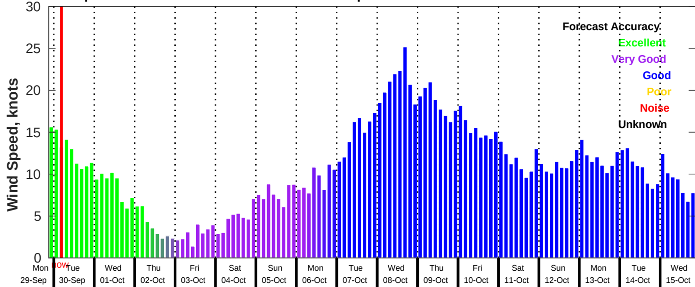
GFS Wind Speed Forecast for NDBC 41040 from 29-Sep-2025 21:00:00 to 15-Oct-2025 21:00:00
