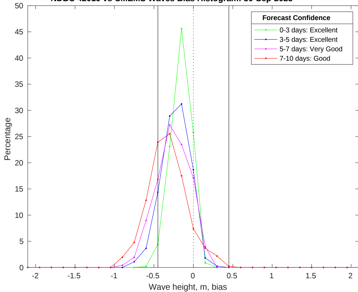
NDBC 42019 vs CMEMS Waves Bias Histogram: 30-Sep-2025
