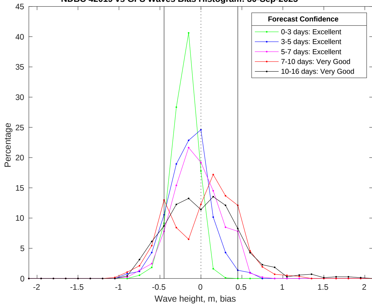
NDBC 42019 vs GFS Waves Bias Histogram: 30-Sep-2025
