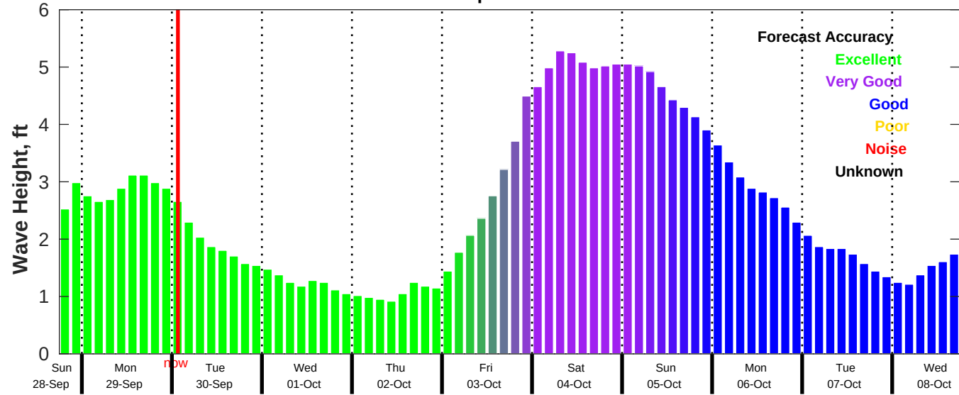
CMEMS Wave Forecast for NDBC 42019 from 28-Sep-2025 18:00:00 to 08-Oct-2025 18:00:00
