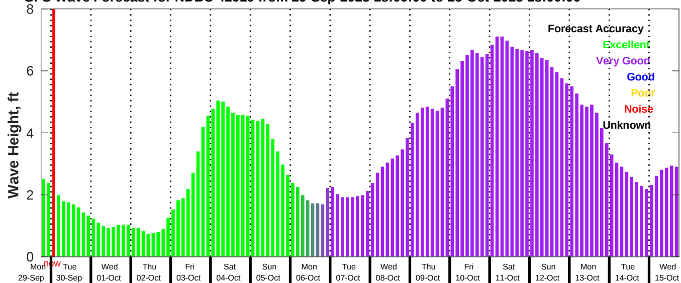
GFS Wave Forecast for NDBC 42019 from 29-Sep-2025 18:00:00 to 15-Oct-2025 18:00:00
