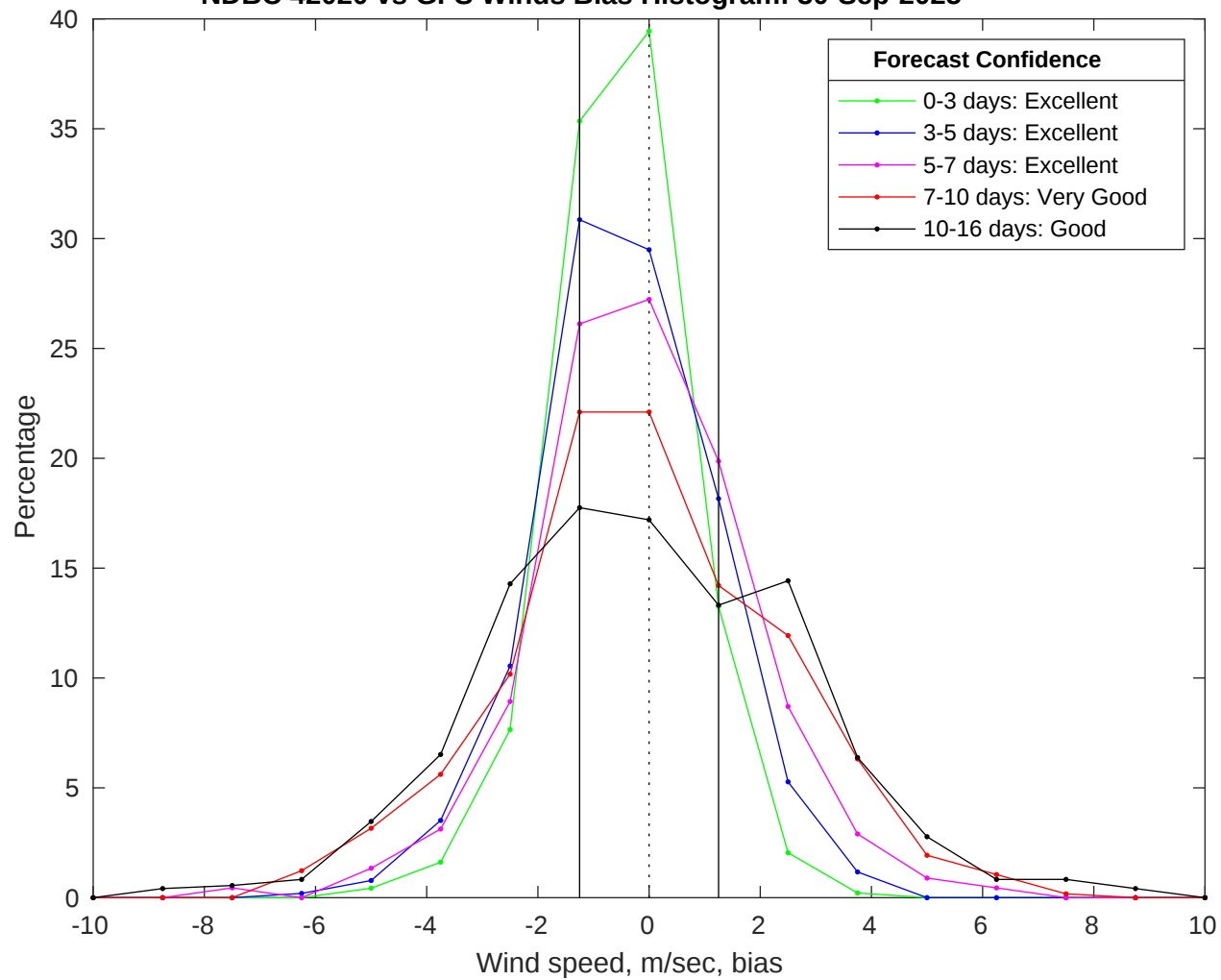
NDBC 42020 vs GFS Winds Bias Histogram: 30-Sep-2025
