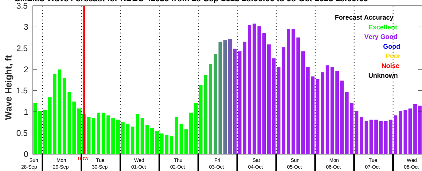
CMEMS Wave Forecast for NDBC 42035 from 28-Sep-2025 18:00:00 to 08-Oct-2025 18:00:00
