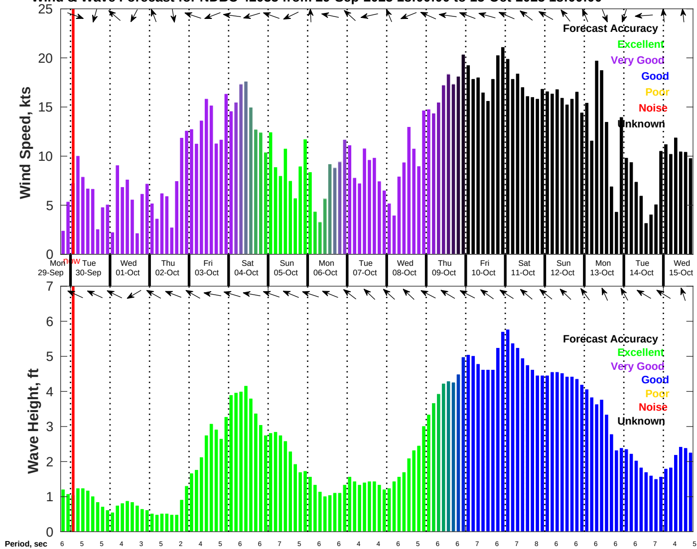
Wind & Wave Forecast for NDBC 42035 from 29-Sep-2025 18:00:00 to 15-Oct-2025 18:00:00
