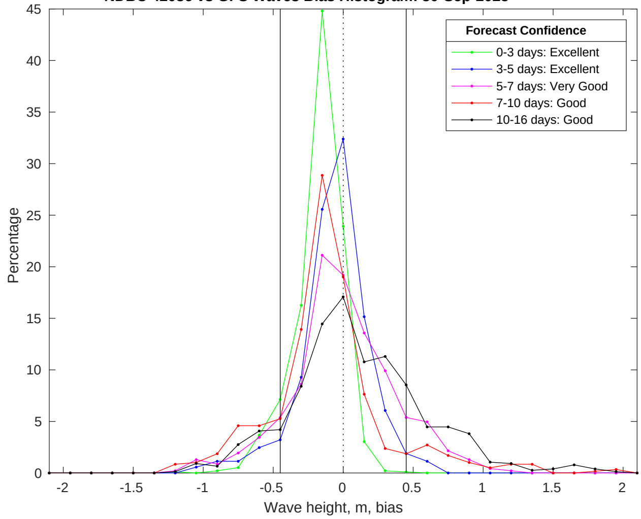
NDBC 42036 vs GFS Waves Bias Histogram: 30-Sep-2025
