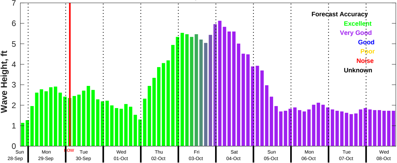
CMEMS Wave Forecast for NDBC 42036 from 28-Sep-2025 19:00:00 to 08-Oct-2025 19:00:00
