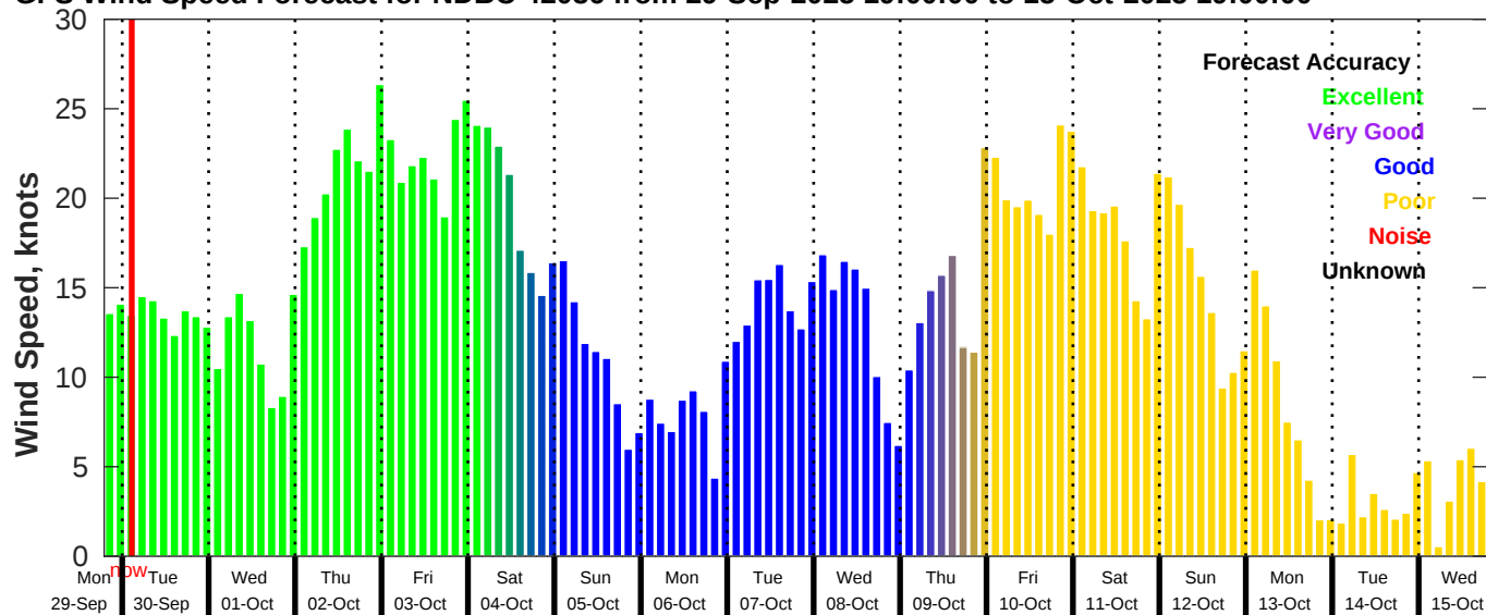
GFS Wind Speed Forecast for NDBC 42036 from 29-Sep-2025 19:00:00 to 15-Oct-2025 19:00:00
