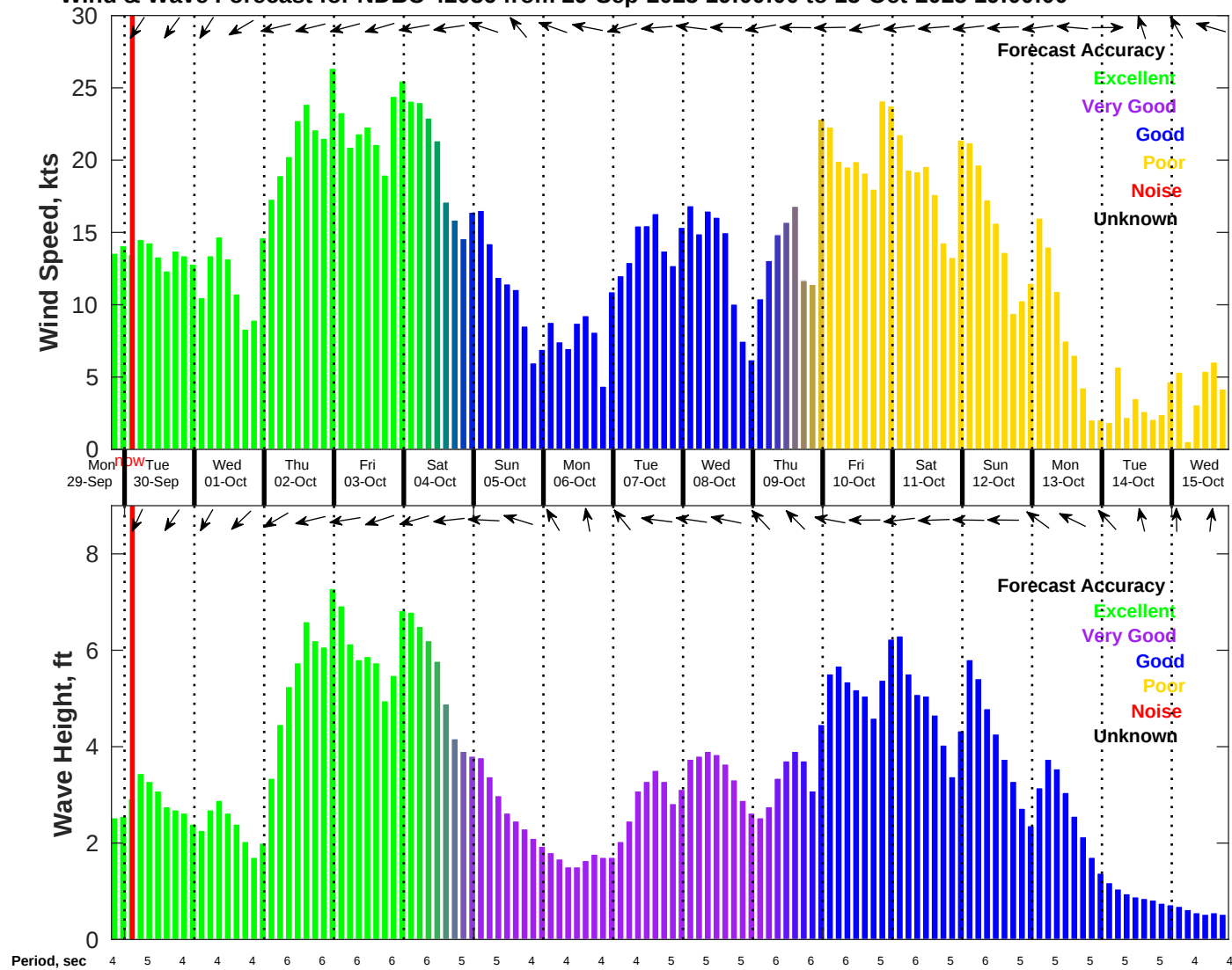
Wind & Wave Forecast for NDBC 42036 from 29-Sep-2025 19:00:00 to 15-Oct-2025 19:00:00
