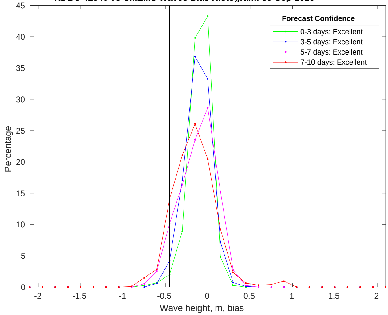
NDBC 42040 vs CMEMS Waves Bias Histogram: 30-Sep-2025
