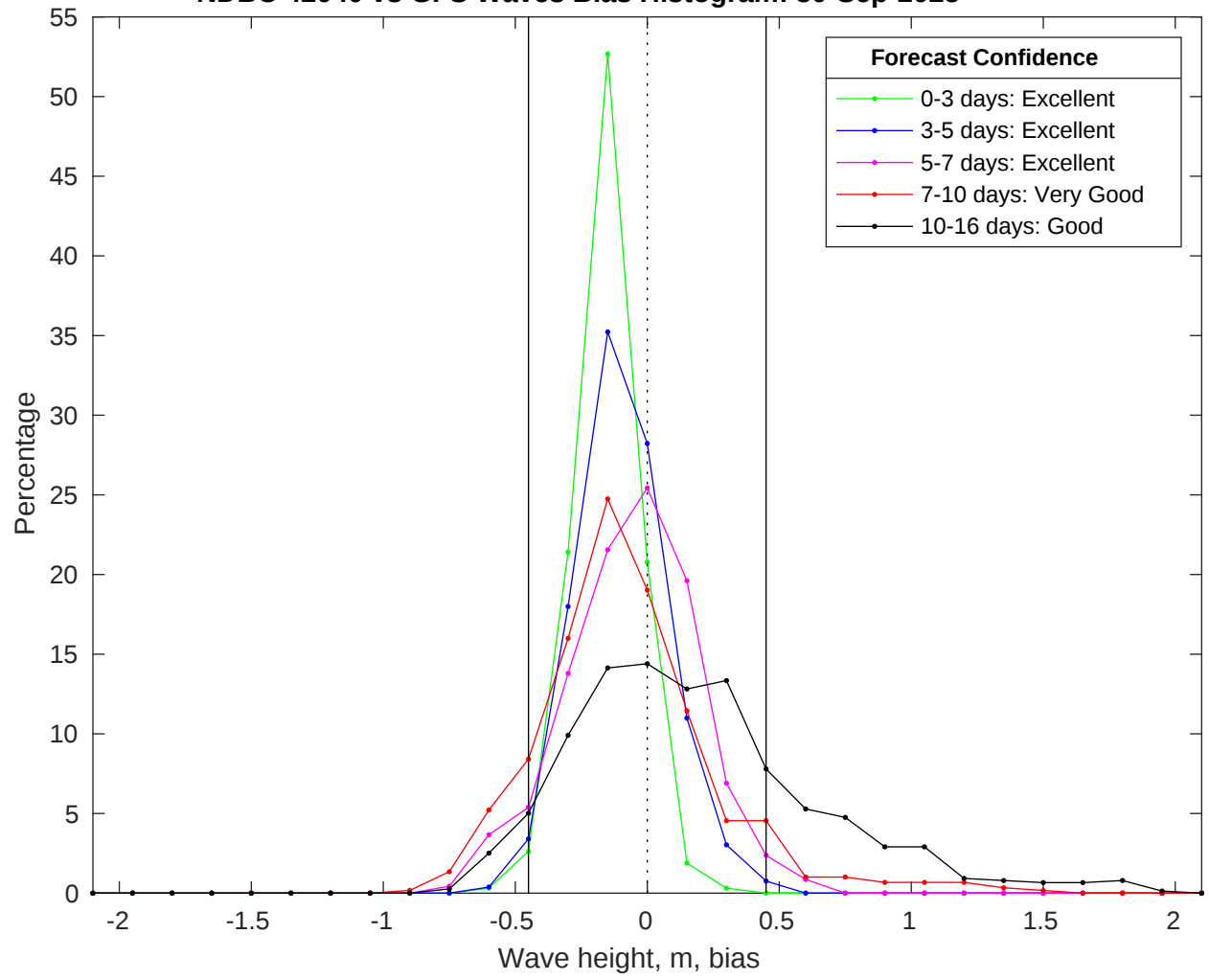
NDBC 42040 vs GFS Waves Bias Histogram: 30-Sep-2025
