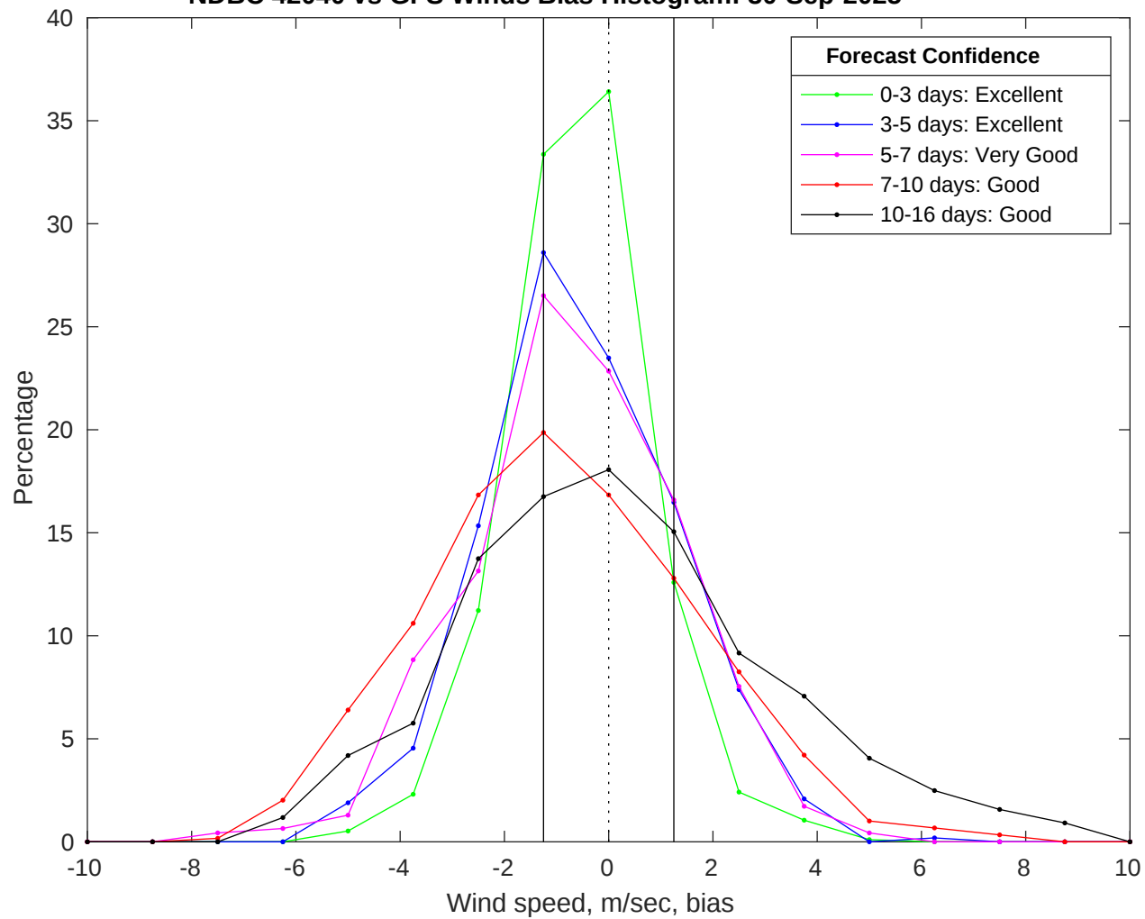
NDBC 42040 vs GFS Winds Bias Histogram: 30-Sep-2025
