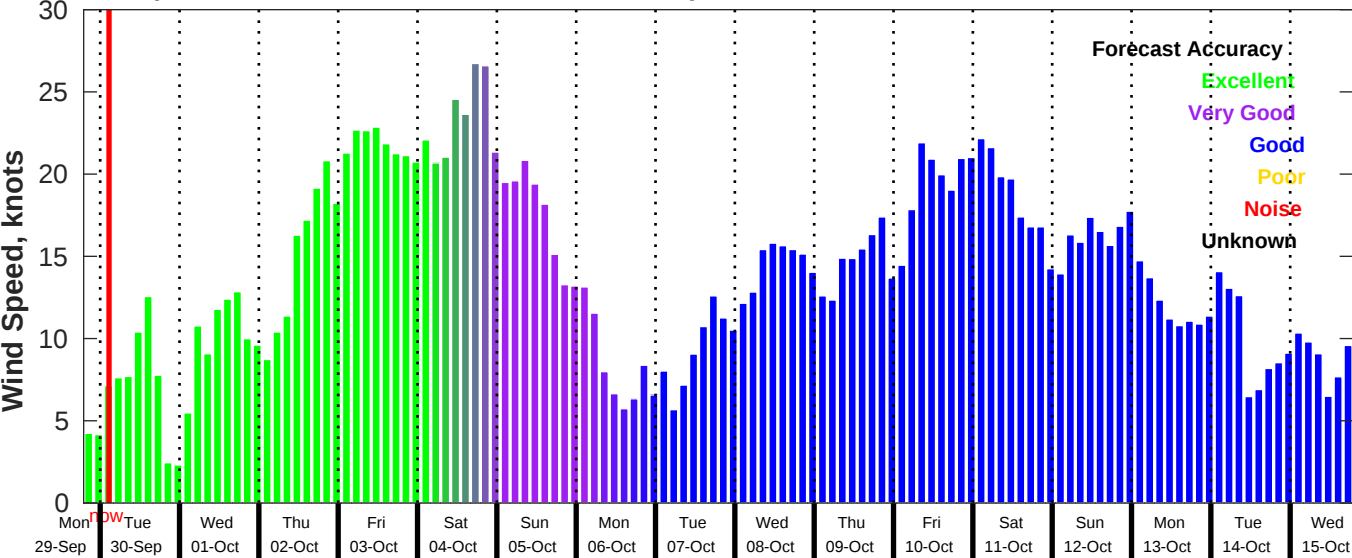
GFS Wind Speed Forecast for NDBC 42040 from 29-Sep-2025 19:00:00 to 15-Oct-2025 19:00:00
