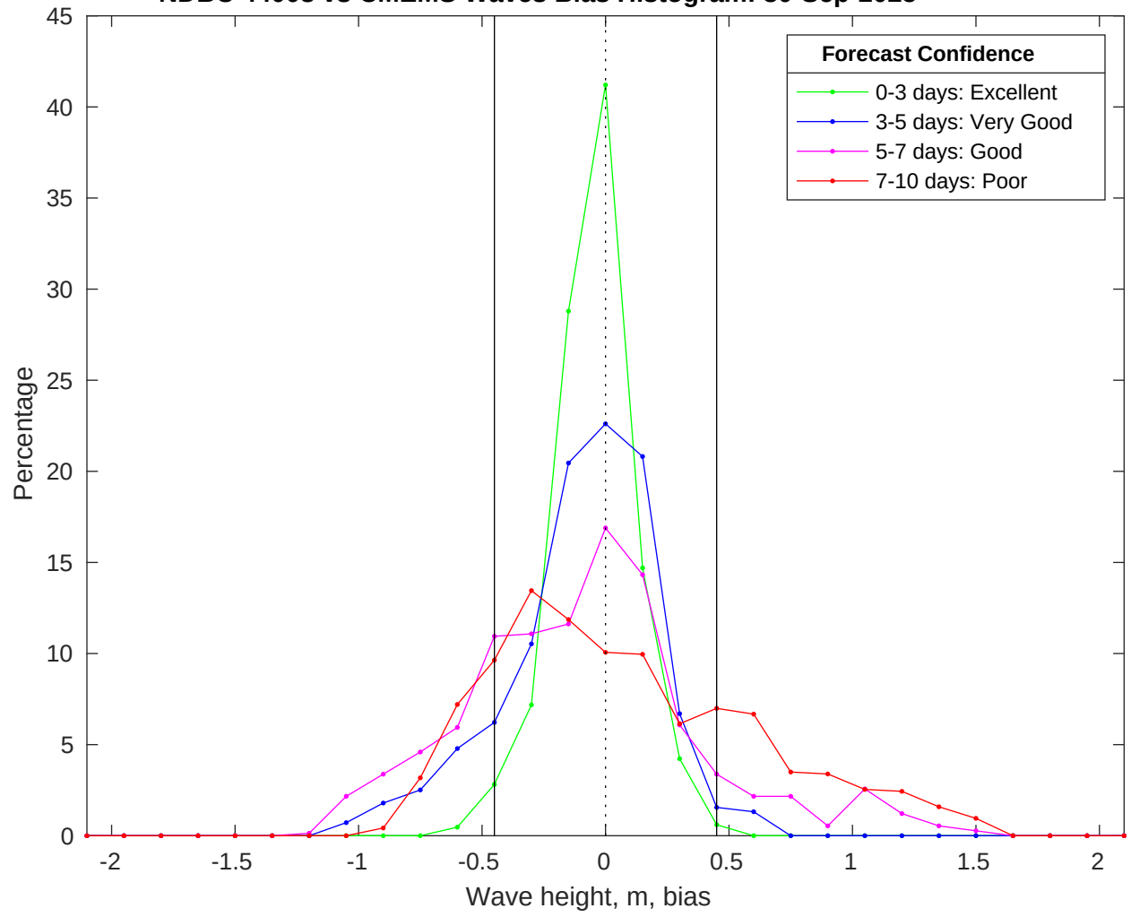
NDBC 44008 vs CMEMS Waves Bias Histogram: 30-Sep-2025
