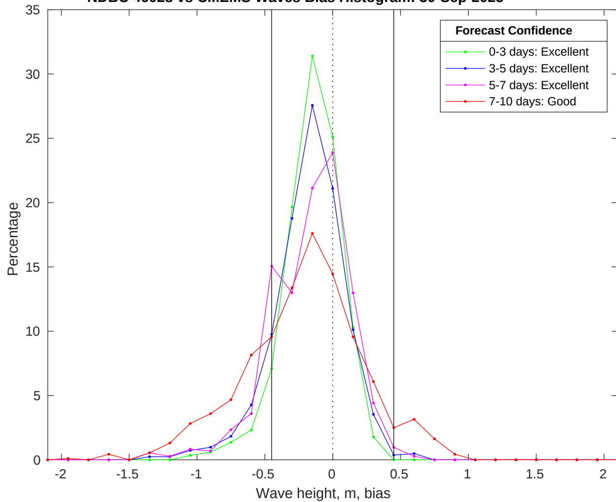
NDBC 46028 vs CMEMS Waves Bias Histogram: 30-Sep-2025
