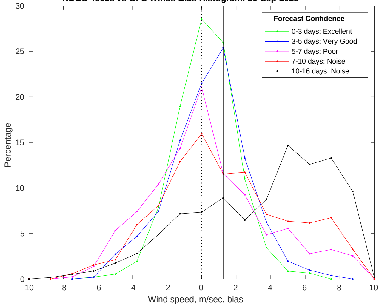
NDBC 46028 vs GFS Winds Bias Histogram: 30-Sep-2025
