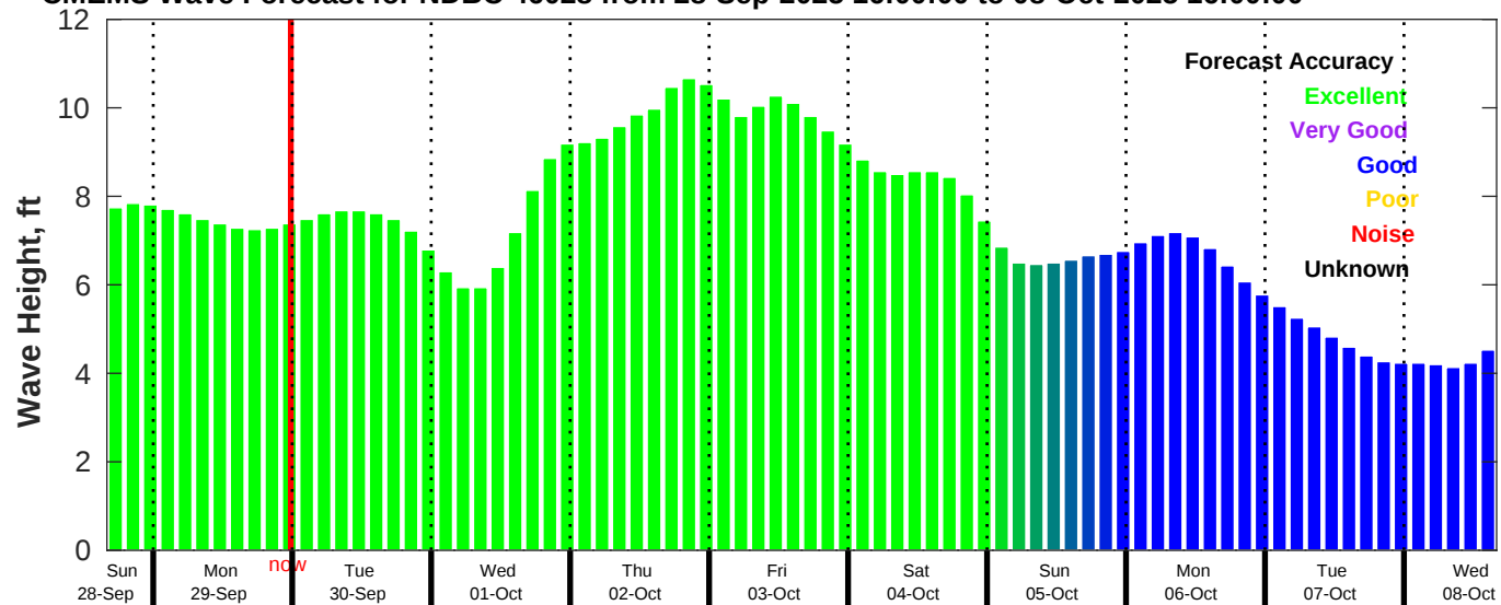
CMEMS Wave Forecast for NDBC 46028 from 28-Sep-2025 16:00:00 to 08-Oct-2025 16:00:00
