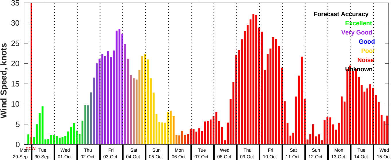
GFS Wind Speed Forecast for NDBC 46028 from 29-Sep-2025 16:00:00 to 15-Oct-2025 16:00:00
