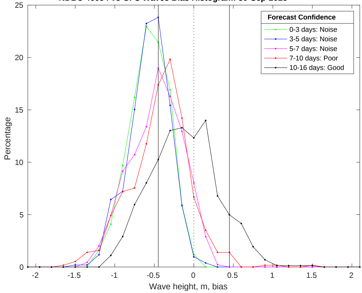
NDBC 46054 vs GFS Waves Bias Histogram: 30-Sep-2025
