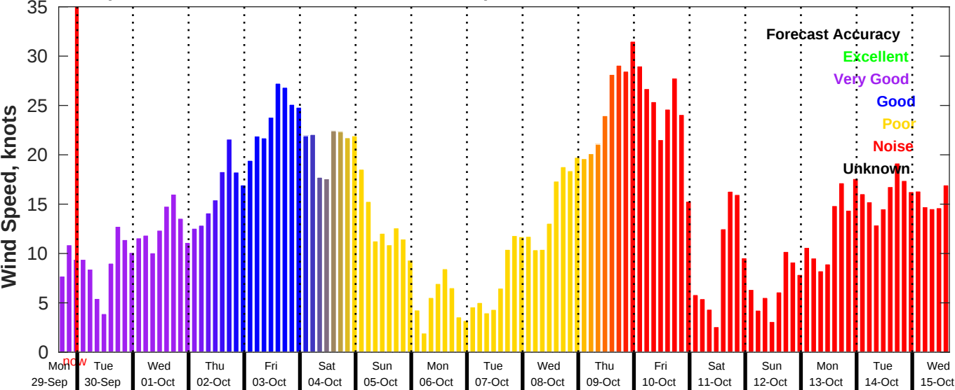
GFS Wind Speed Forecast for NDBC 46054 from 29-Sep-2025 16:00:00 to 15-Oct-2025 16:00:00
