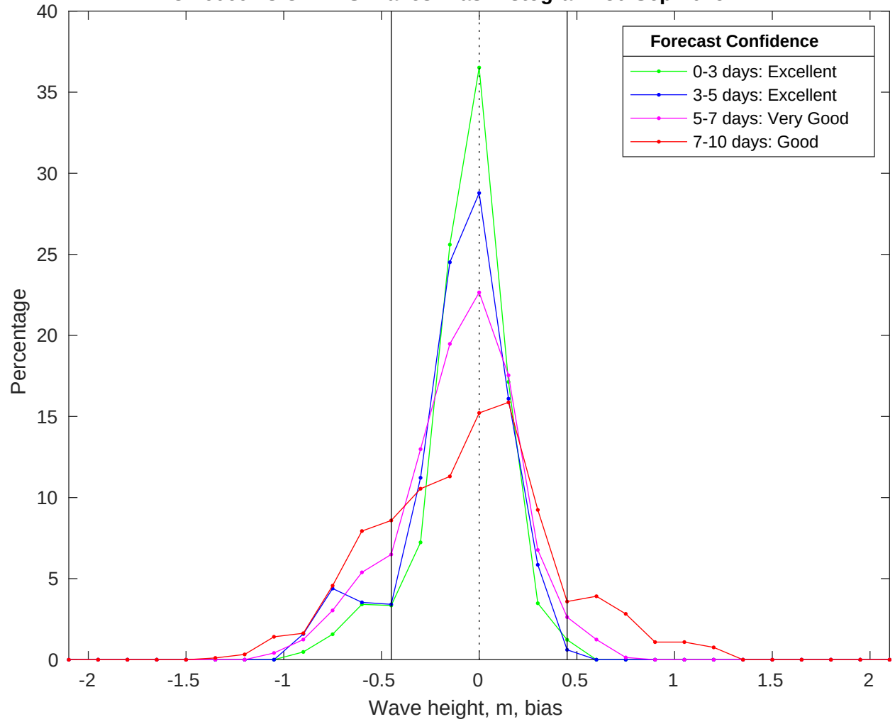
NDBC 46069 vs CMEMS Waves Bias Histogram: 30-Sep-2025
