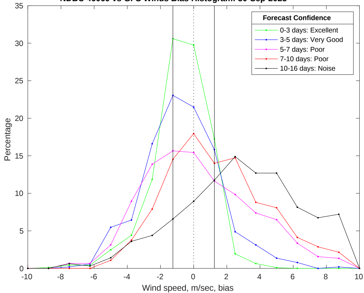
NDBC 46069 vs GFS Winds Bias Histogram: 30-Sep-2025
