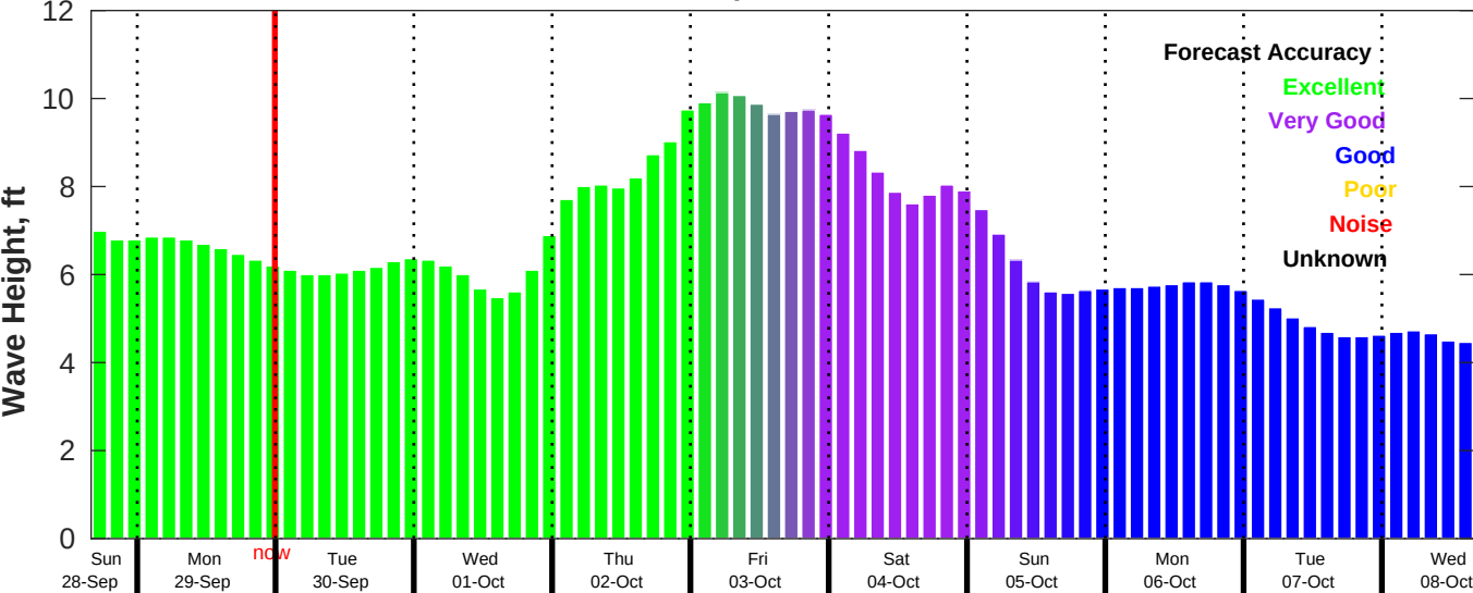
CMEMS Wave Forecast for NDBC 46069 from 28-Sep-2025 16:00:00 to 08-Oct-2025 16:00:00
