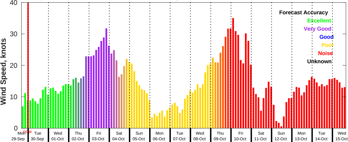
GFS Wind Speed Forecast for NDBC 46069 from 29-Sep-2025 16:00:00 to 15-Oct-2025 16:00:00
